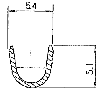
SECT. B-B
