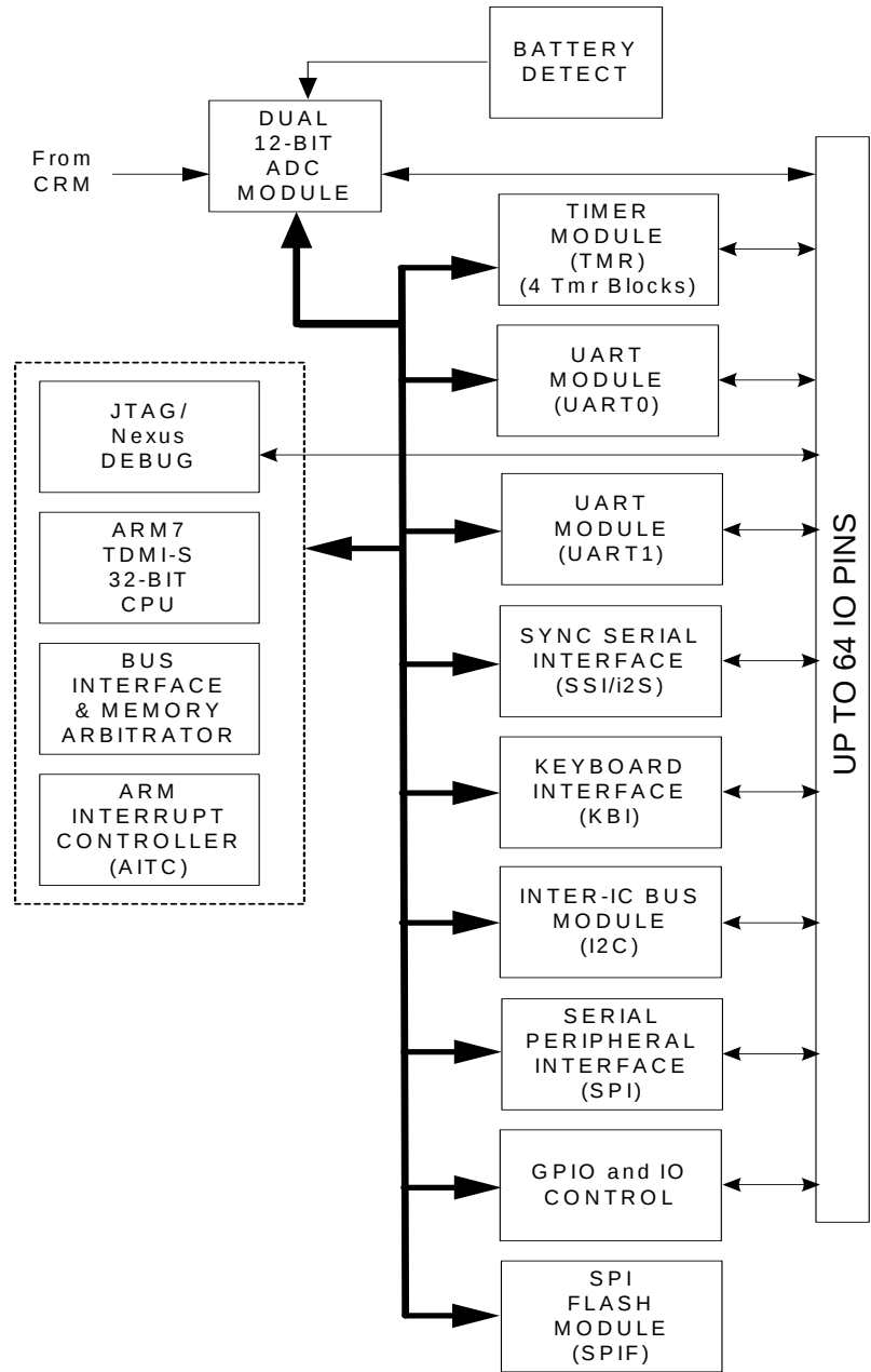
Figure 6. MCU Peripherals
