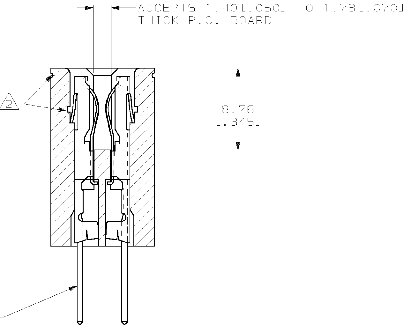
SECTION Z-Z
