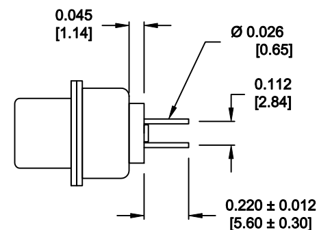
SIGNAL CONTACTS
