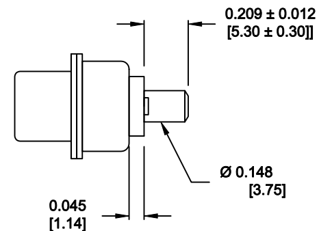
POWER CONTACTS
