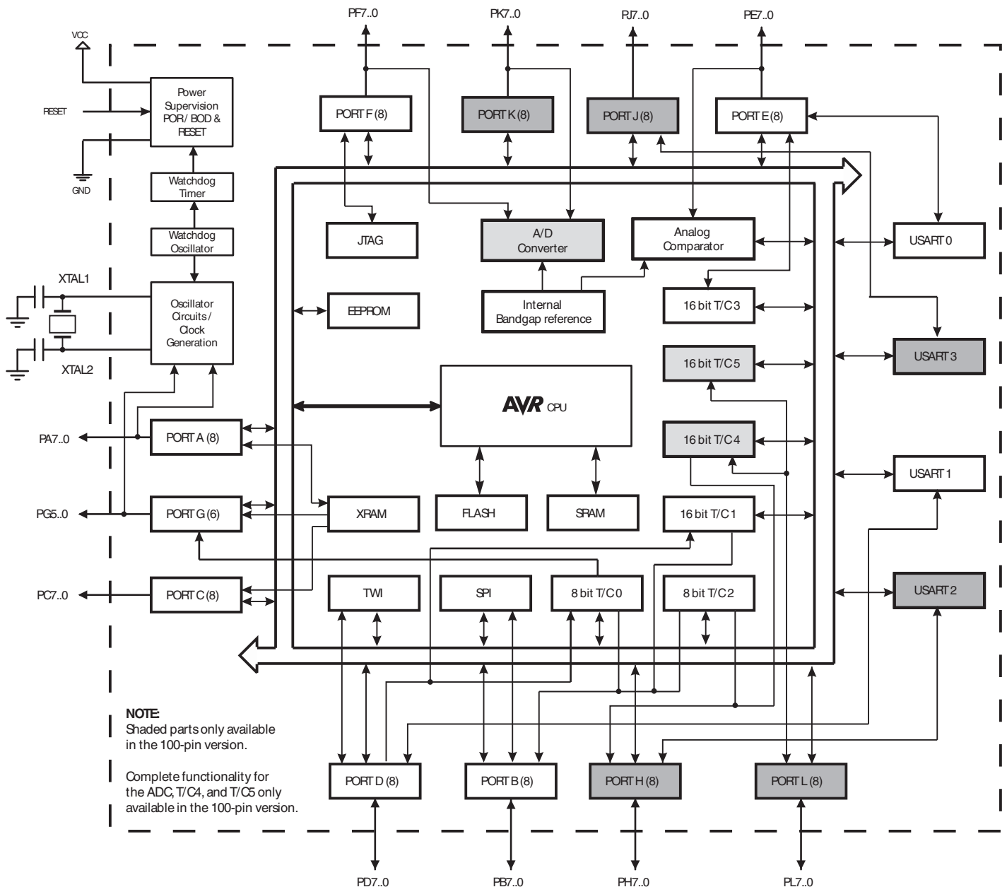
Figure 2-1. Block Diagram
