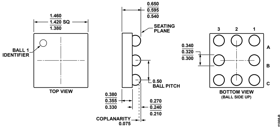
Figure 54. 8-Ball Wafer Level Chip Scale Package [WLCSP] (CB-8-2) Dimensions shown in millimeters
