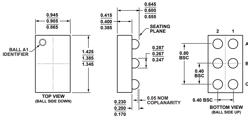
Figure 52. 6-Ball Wafer Level Chip Scale Package [WLCSP] (CB-6-7) Dimensions shown in millimeters
