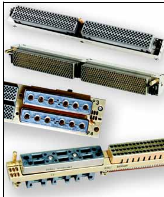
From top to bottom: Staggered Grid, 2 Bay LRM; GEN-X Grid, 2 Bay LRM; LRM inserts with RADSOX contacts; LRM insert with MT ferrule fiber optics and brush contacts in a Differential Pair insert.
