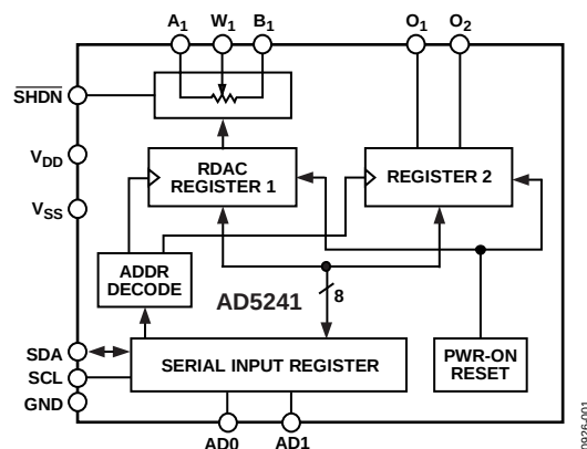
Figure 1. AD5241 Functional Block Diagram
