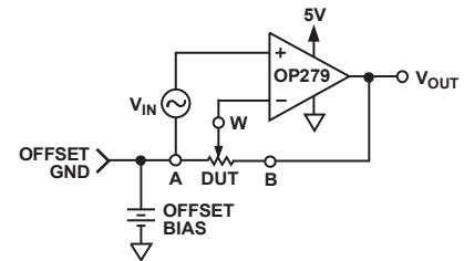
Figure 27. Noninverting Gain
