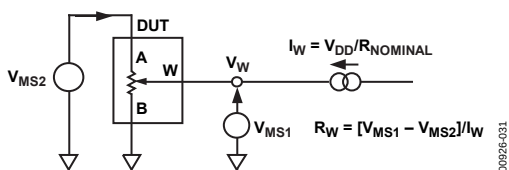
Figure 24. Wiper Resistance
