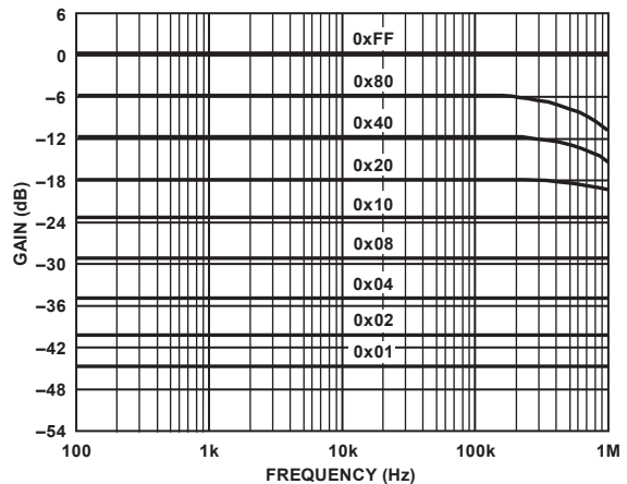
Figure 19. AD5242 10kΩ Gain vs. Frequency vs. Code
