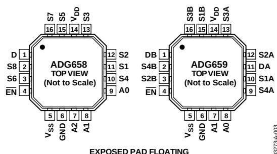
Figure 3. 16-Lead, 4 mm × 4 mm LFCSP Pin Configuration
