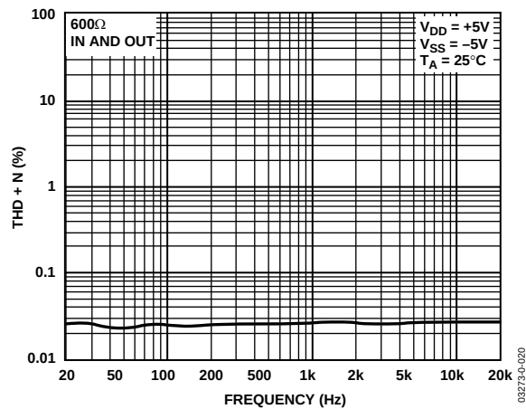
Figure 18. THD + Noise
