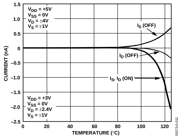
Figure 10. Leakage Current vs. Temperature (Single Supply)
