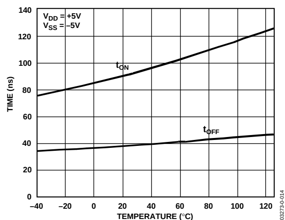
Figure 12. t_{ON}/t_{OFF} Times vs. Temperature (Dual Supply)
