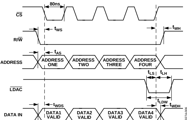
Figure 6. Double-Buffer Mode
