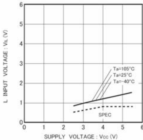
Figure 2. L input voltage V_{IL} (CS,SK,DI)
