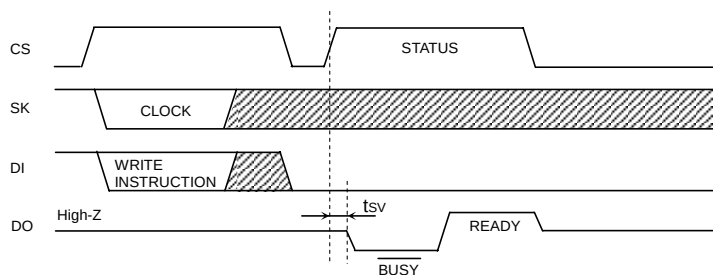
Figure 46. R/B status output timing chart
