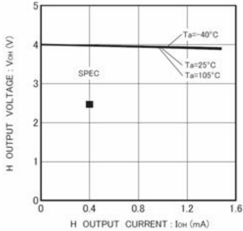
Figure 6. H output voltage V_{OH} - I_{OH} ( V_{CC} = 4.0\text{V} )
