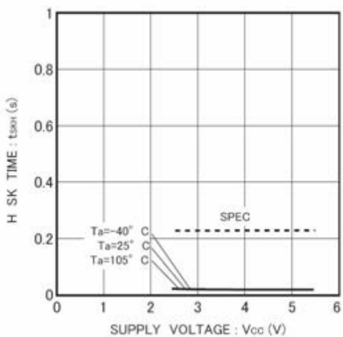
Figure 14. SK high time t_{SKH}
