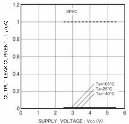
Figure 8. Output leak current I_{LO} (DO)
