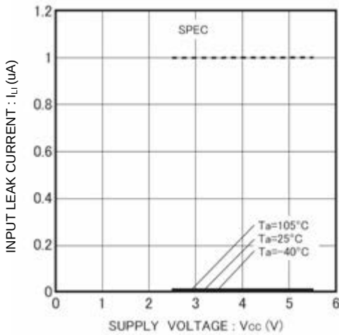
Figure 7. Input leak current I_{LI} (CS, SK, DI)
