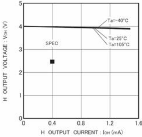
Figure 6. H output voltage V_{OH} - I_{OH} ( V_{CC}=4.0\text{V} )
