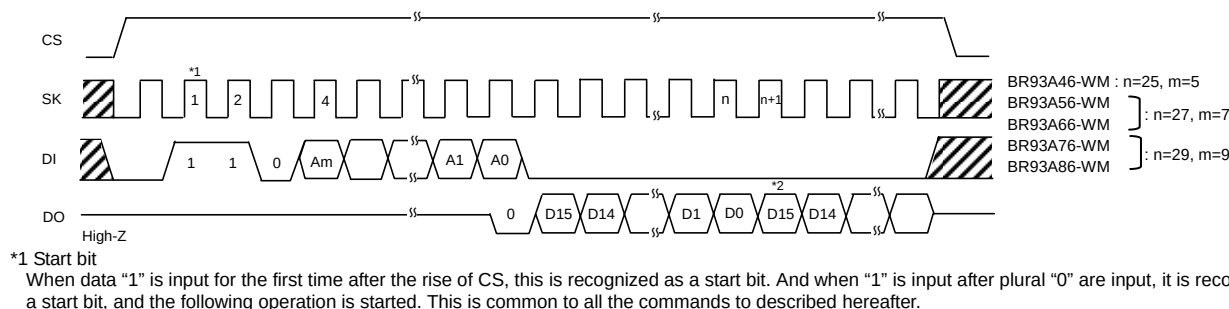
Figure 27. Read cycle
