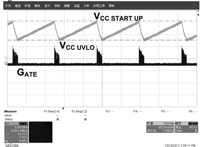
Figure 14 UVLO
