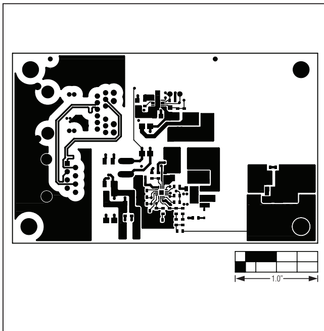
Figure 3. MAX5974E EV Kit PCB Layout—Component Side
