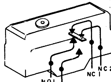
CIRCUIT DIAGRAM
