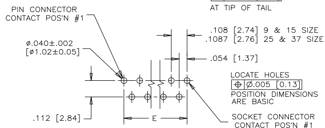
RECOMMENDED P.C.B. LAYOUT (COMPONENT SIDE OF BOARD)
