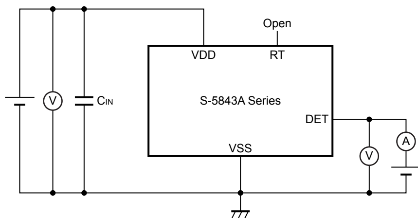
Figure 6 Test Circuit 2
