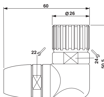
Dimensional drawing
