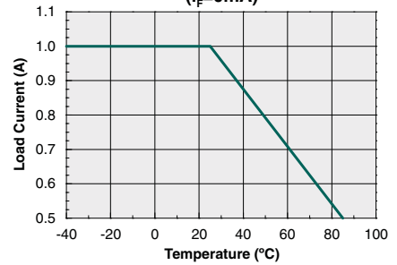
Maximum Load Current vs. Temperature AC/DC Configuration ( I_F=0mA )
