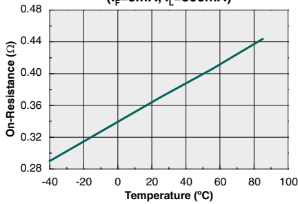
Typical On-Resistance vs. Temperature AC/DC Configuration ( I_F=0mA, I_L=500mA )
