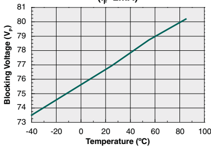
Typical Blocking Voltage vs. Temperature ( I_F=2mA )
