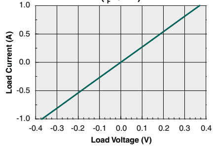
Typical Load Current vs. Load Voltage AC/DC Configuration ( I_F=0mA )
