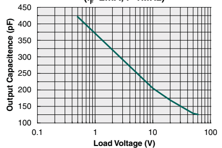
Output Capacitance vs. Load Voltage ( I_F=2mA, f=1MHz )
