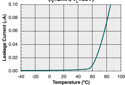
Typical Leakage Current vs. Temperature ( I_F=2mA, V_L=60V )
