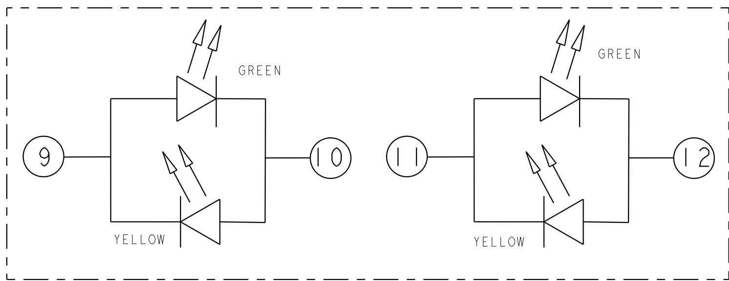
BI-COLOR LED
