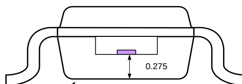
END VIEW
