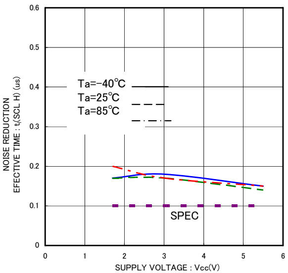
Fig.28 Noise reduction effective time t_i(SCL:H)
