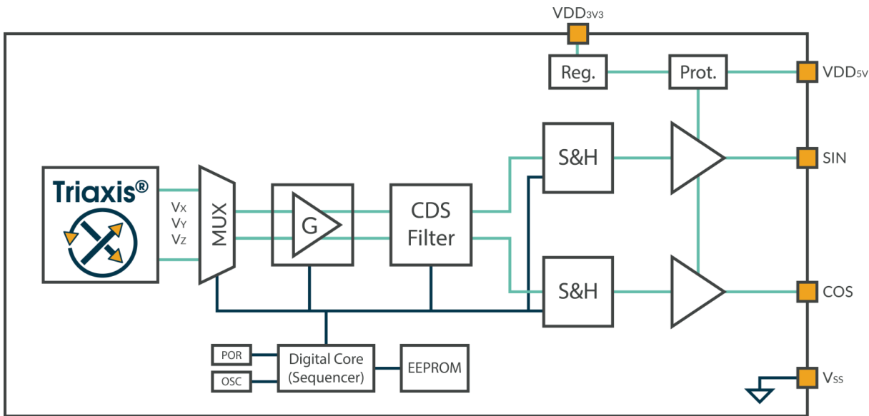
Figure 3: Functional Diagram
