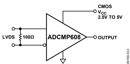
Figure 13. LVDS-to-CMOS Receiver
