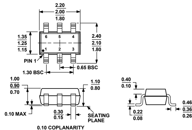
COMPLIANT TO JEDEC STANDARDS MO-203-AB Figure 14. 6-Lead Thin Shrink Small Outline Transistor Package (SC70) (KS-6) Dimensions shown in millimeters
