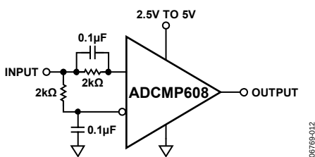
Figure 12. Self-Biased, 50% Slicer
