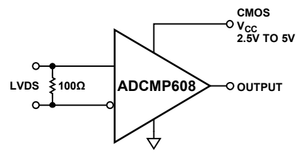
Figure 13. LVDS-to-CMOS Receiver
