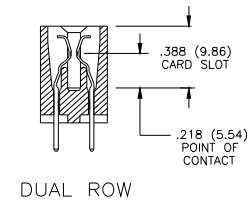
DUAL ROW BETWEEN CONTACT POLARIZING KEY P/N 306-240-318
