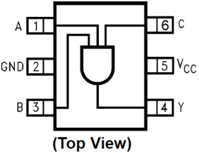
Pin One Orientation Diagram
