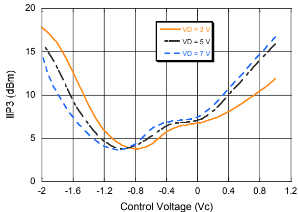
Input IP3 @ 10 GHz
