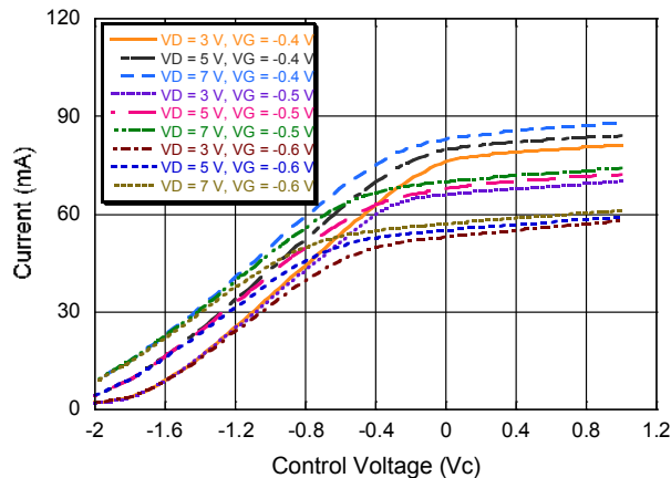
Current @ 10 GHz
