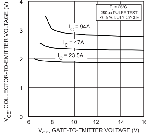
FIGURE 5, On State Voltage vs Gate-to-Emmitter Voltage
