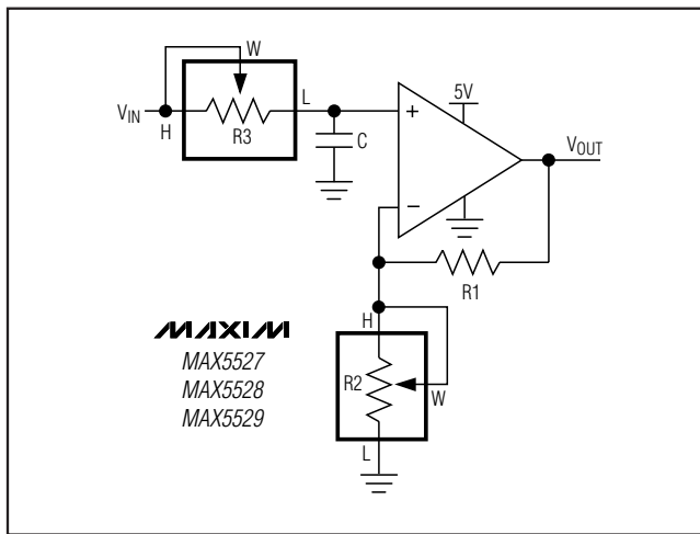
Figure 9. Programmable Filter
