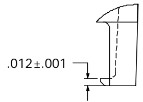
DETAIL A SCALE= 6X
