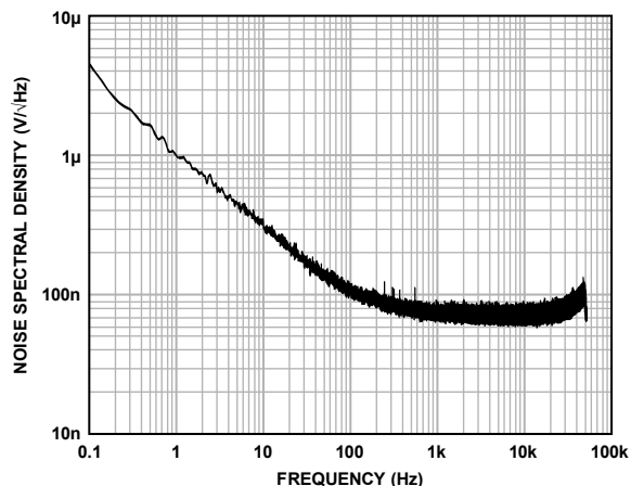
Figure 52. VREF_IO Output NSD vs. Frequency
