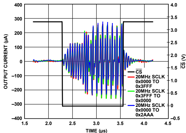
Figure 54. Digital Feedthrough
