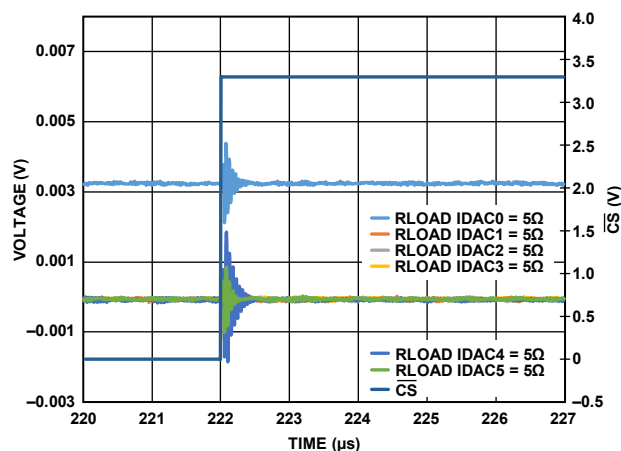
Figure 56. Analog Crosstalk
