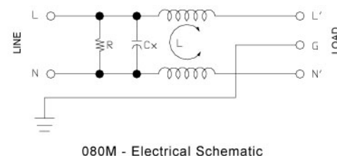
080M - Electrical Schematic
