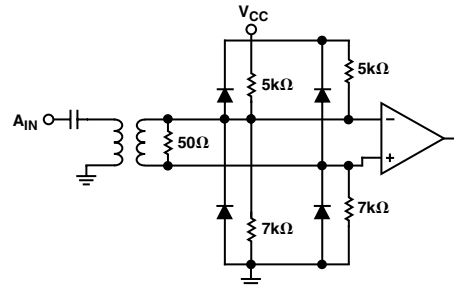
Figure 5. Equivalent Analog Input Circuit
