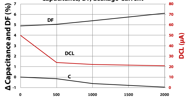
Life Test 105 °C, Full Load, 330 μF, 400 Vdc Capacitance, DF, Leakage Current
