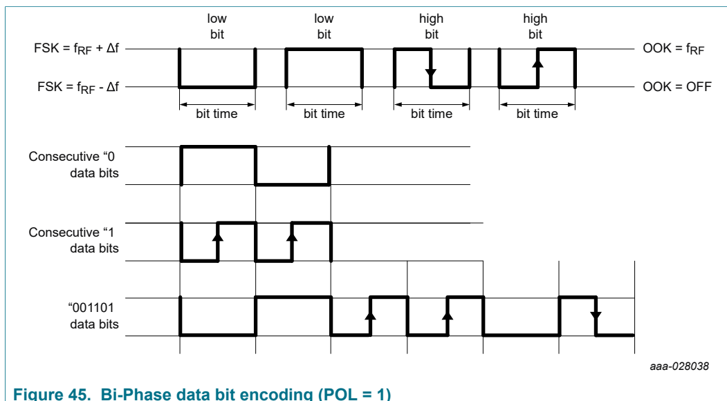
Figure 45. Bi-Phase data bit encoding (POL = 1)
