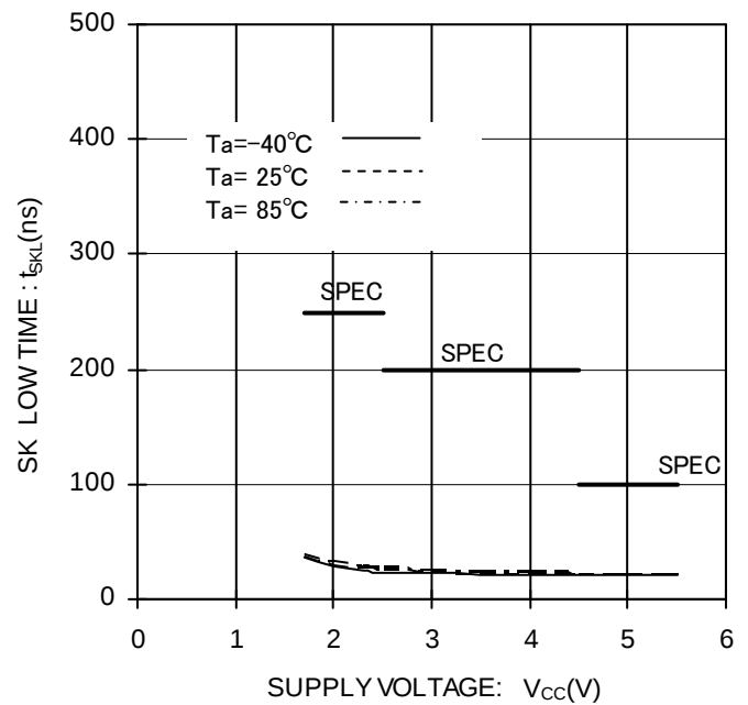
Figure 23. SK Low Time vs Supply Voltage
