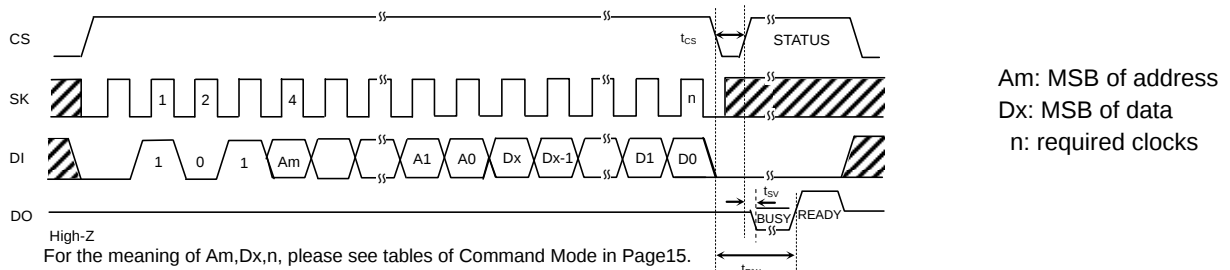
Figure 36. Write Cycle
