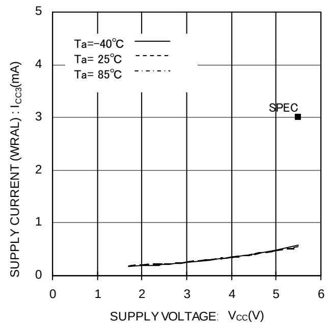
Figure 19. Supply Current (WRAL) vs Supply Voltage ( f_{SK}=3\text{MHz} )
