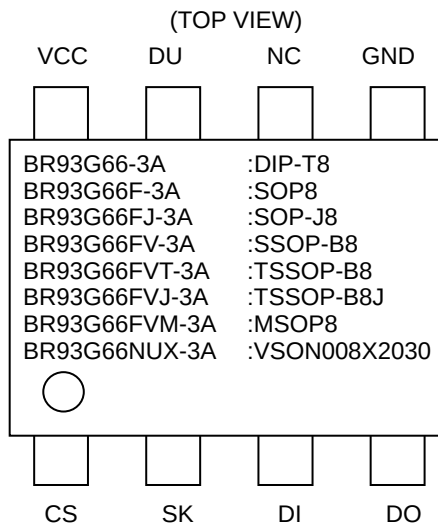
Figure 3. Pin Configuration
