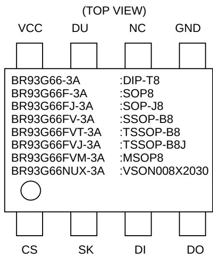
Figure 3. Pin Configuration
