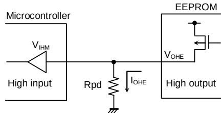
Figure 47. DO Pull Down Resistance
