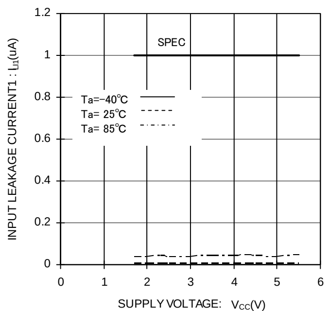
Figure 11. Input Leakage Current (SK) vs Supply Voltage
