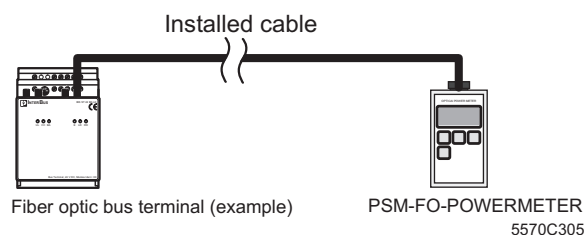
Figure 50 Power measurement of fiber optic cables
