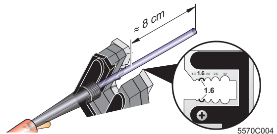
Figure 36 Stripping the individual wires
