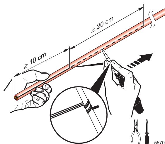
Figure 32 Tearing open the cable sheath
