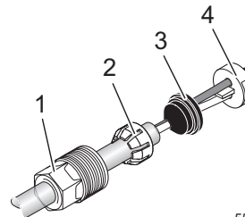
Figure 25 Individual parts
