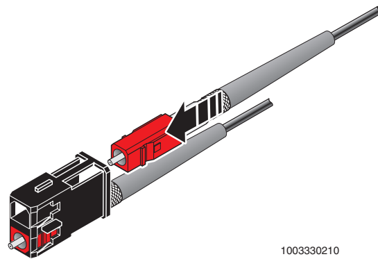
Figure 49 Assembling the SC-RJ connector
